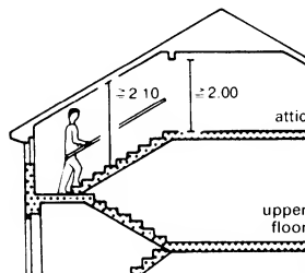
⑧ Laying the rafters and beams parallel to the stairs saves space and avoids the need for expensive alterations
